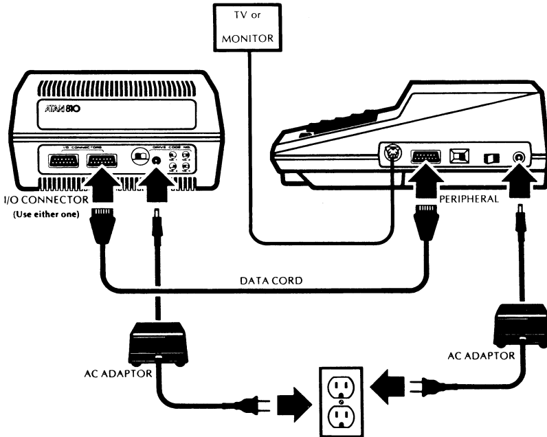
EQUIPMENT HOOK-UP
